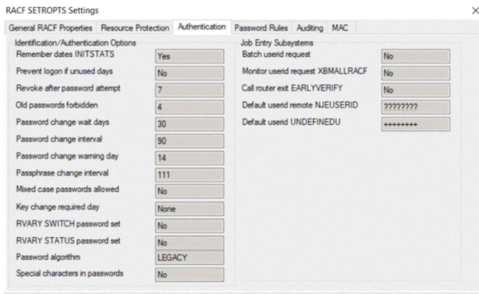
Figure 26. RACF SETROPTS Settings - Authentication tab
