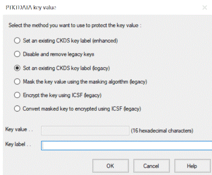
Figure 83. PTKTDATA key value dialog
