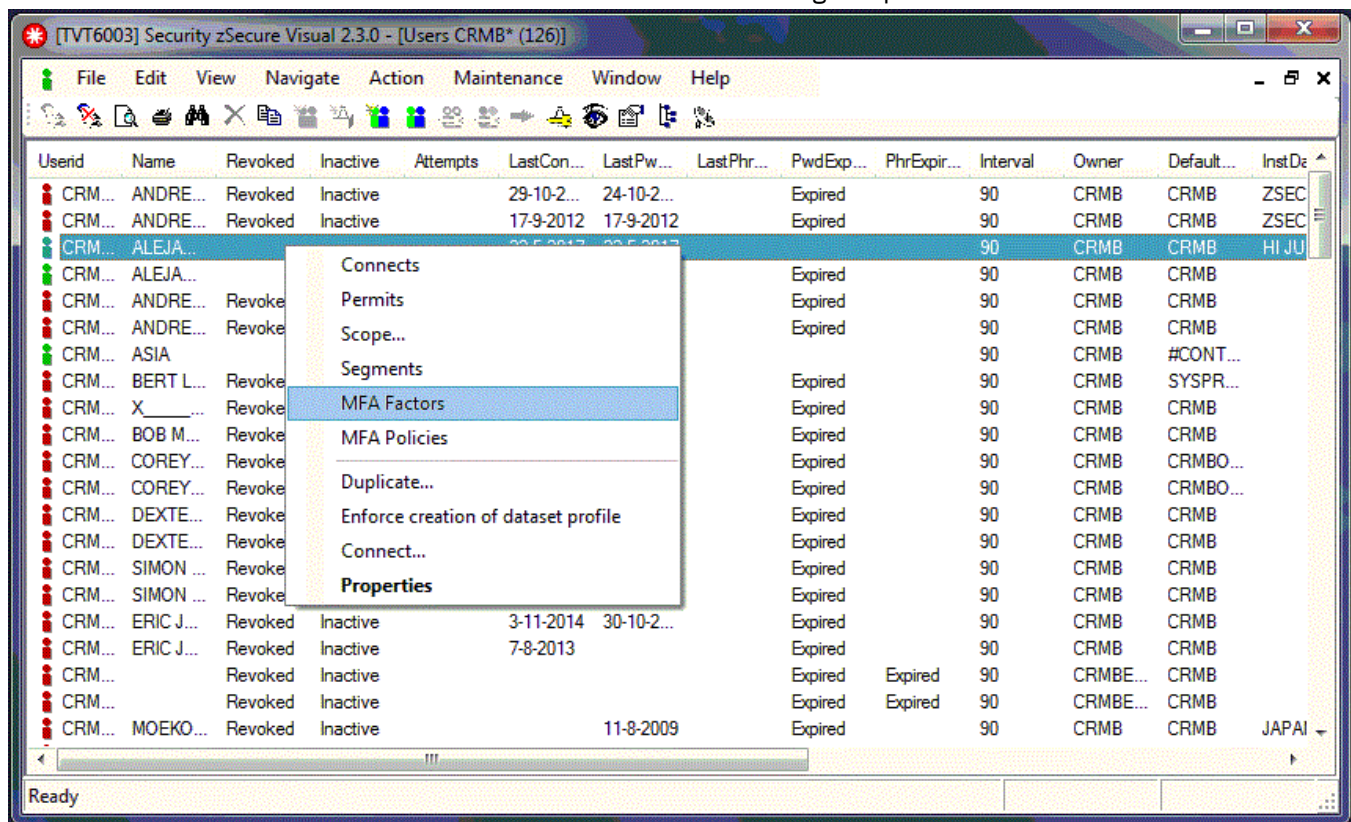
Figure 44. MFA User table
