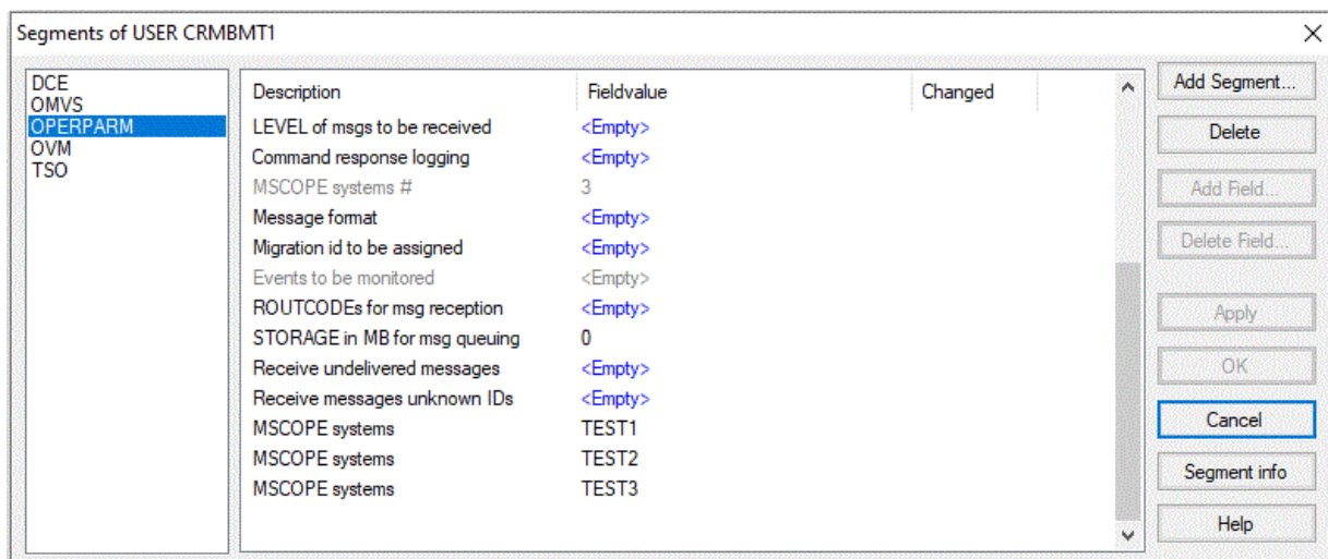
Figure 80. Segment Detail Window
