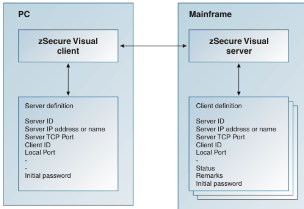
Figure 84. Server and client definitions needed for communication between the server and a client
